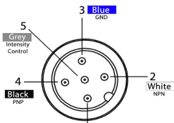
Pin layout for light (Male Connector)
