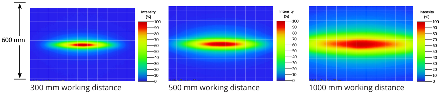
Line (10° x 50°) beam patterns Grid set to 75 mm
