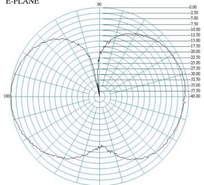
Antenna Pattern
