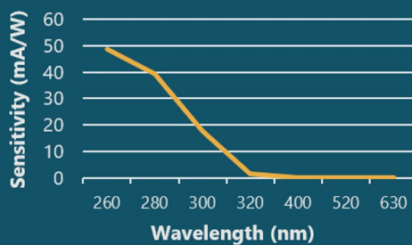
Photocathode Sensitivity
